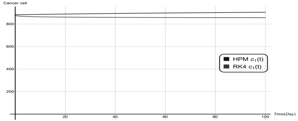
Fig. 5(e): Comparison of HPM and RK4 results for c_1(t) over 0-100 days, with the FO parameter \alpha = 0.45 .
